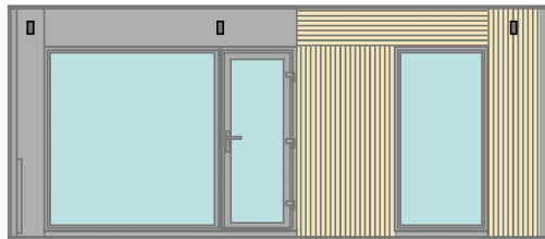
Front facade
