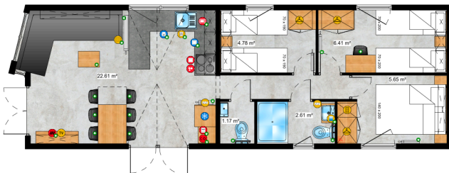
3. 12,46m x 4m / 41ft x 13ft
