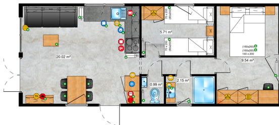
12. 9,6m x 4m / 31ft x 13ft
